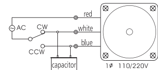
Wiring Diagram
