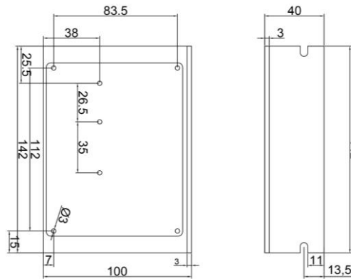
接口定义 (CONNECTOR IDENTIFICATION)
