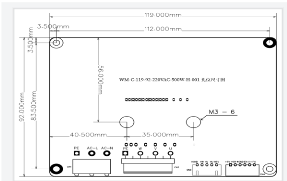
PCB尺寸圖mm (PCB DRAWING)
