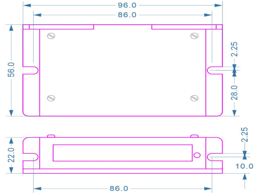
散热片尺寸图 (Casing DRAWING)
