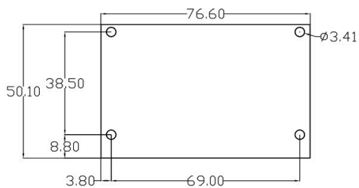
PCB尺寸图 (PCB DRAWING)
