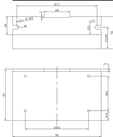
散热器壳尺寸图 (HEAT SINK DRAWING)
