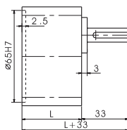
Detailed gearbox output shaft dimension
