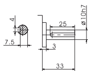
Detailed gearbox output shaft dimension
