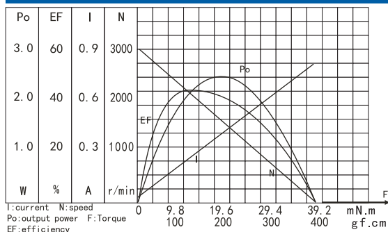
ZY31243000CHARAC TERISTICS
