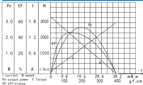
ZY31123000CHARAC TERISTICS
