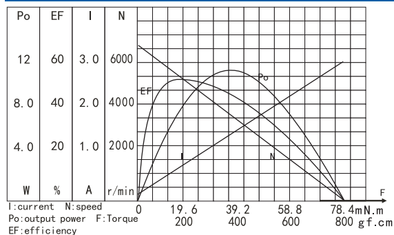
ZY31246000CHARAC TERISTICS
