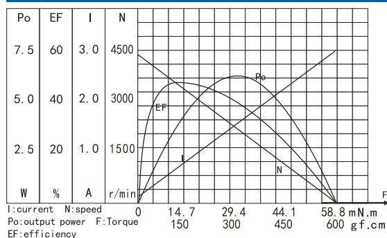
ZY31124500CHARAC TERISTICS
