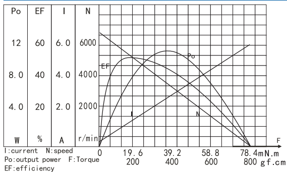
ZY31126000CHARAC TERISTICS
