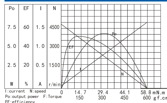
ZY31244500CHARAC TERISTICS
